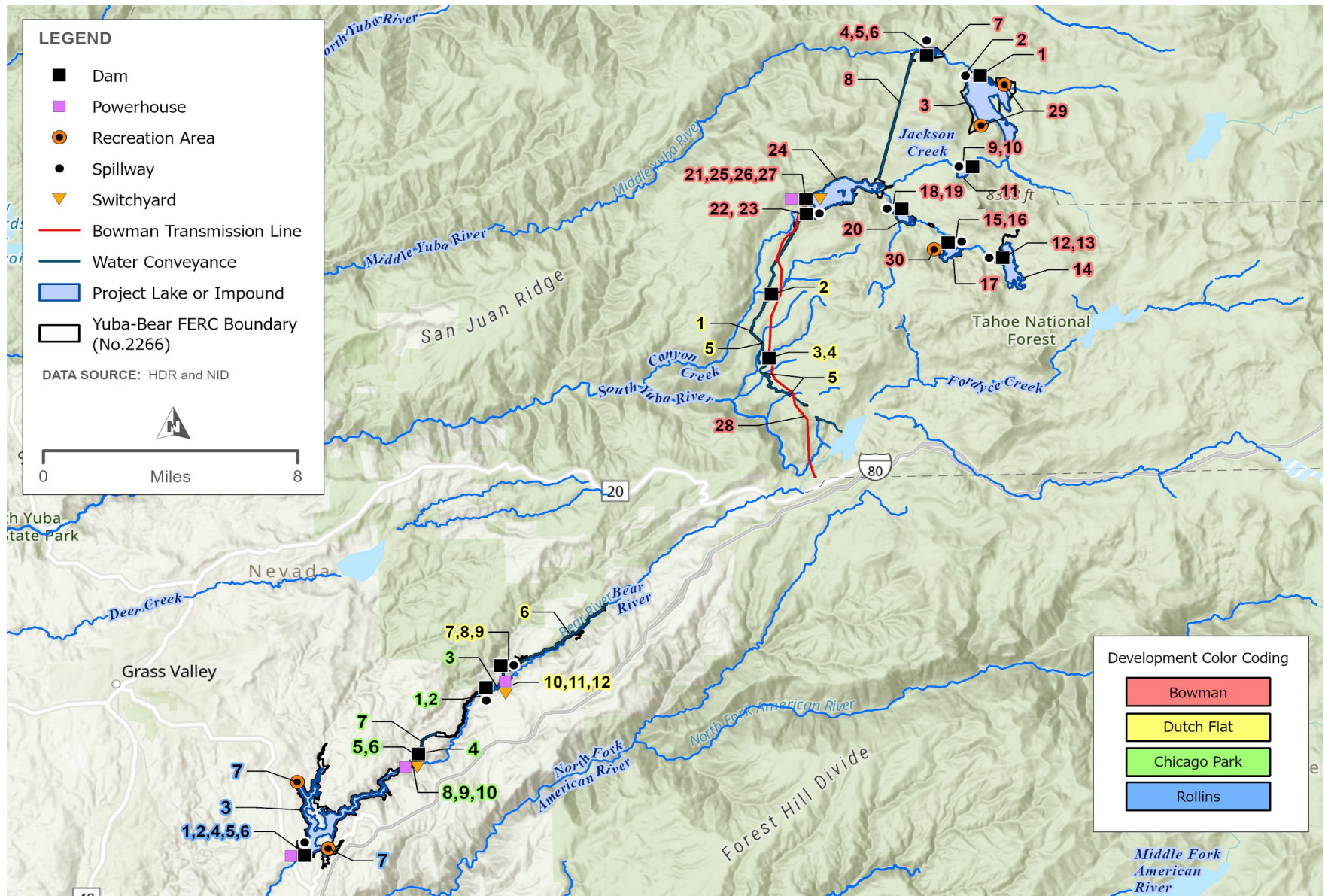
Figure 3-1. Yuba-Bear Hydroelectric Project Facilities.
