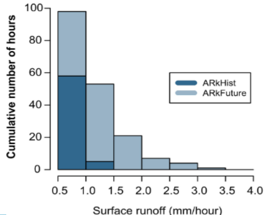
E 1-hour runoff rates, Sacramento Basin
